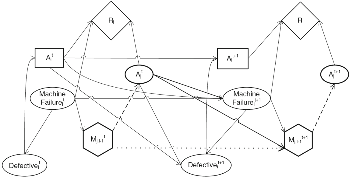
Figure 6.6: Level 1 I-DID of agent i for the multiagent MM problem. The hexagonal model node contains M level 0 DIDs of agent j . At horizon 1, the models of j are IDs [14].
