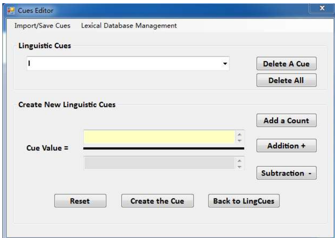
Figure 4.8: Cues Editor
