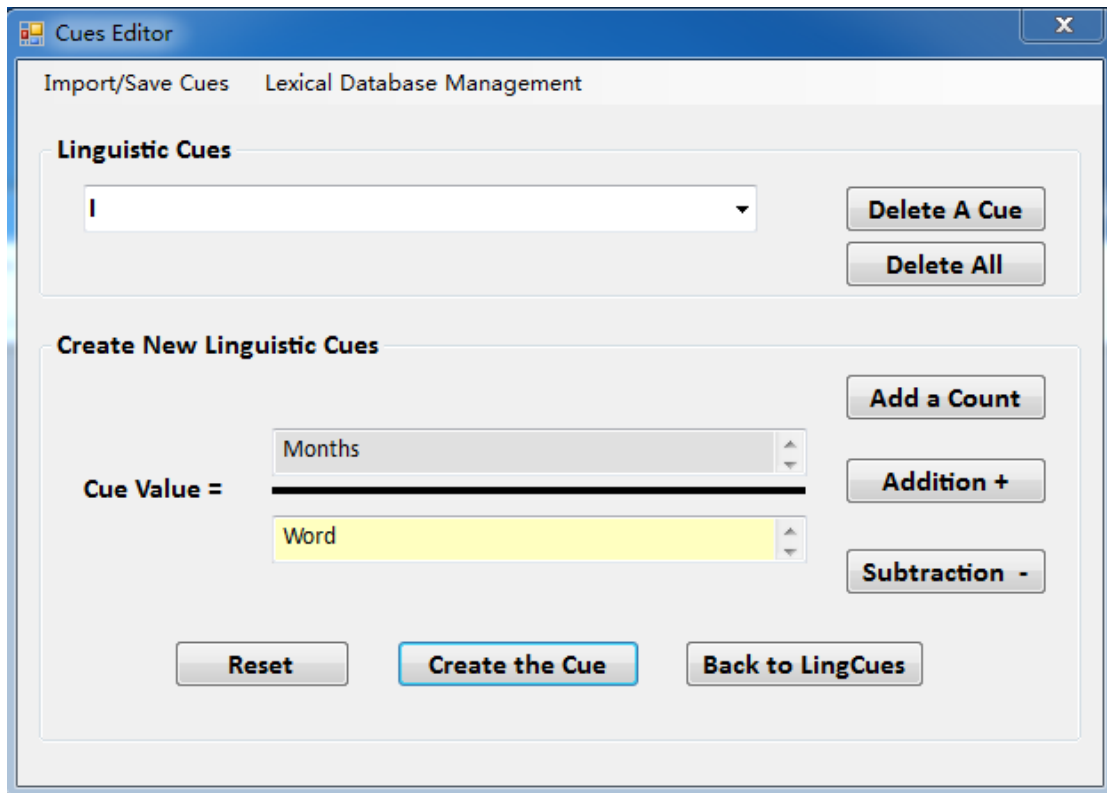
Figure 4.13: The cue value equation in Cues Editor
