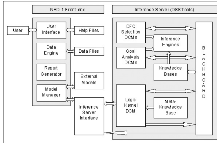
Figure 1.1: NED-1 Architecture
