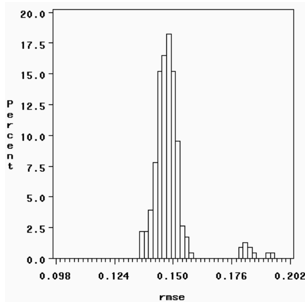
Figure 6.8: Histogram of RMS error values from all experiments.
