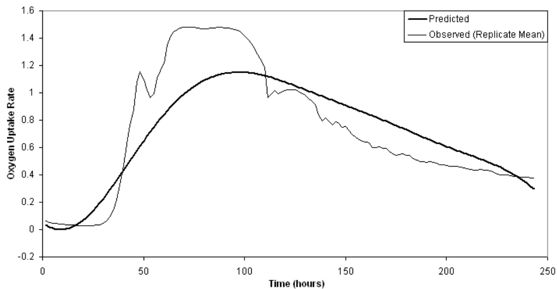
Figure 6.5: Best FIS applied to validation set, moisture 60%
