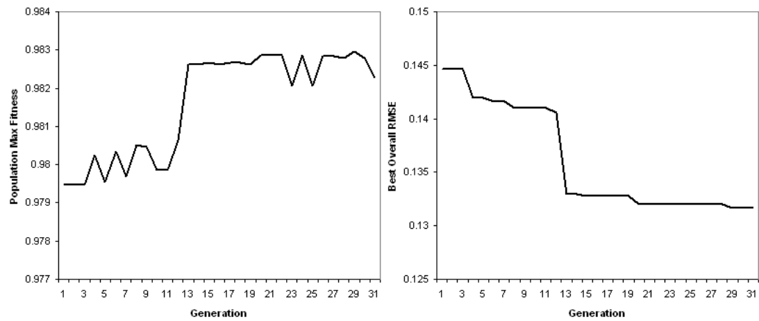
Figure 6.7: Population maximum fitness (left) and overall best RMS error (right).
