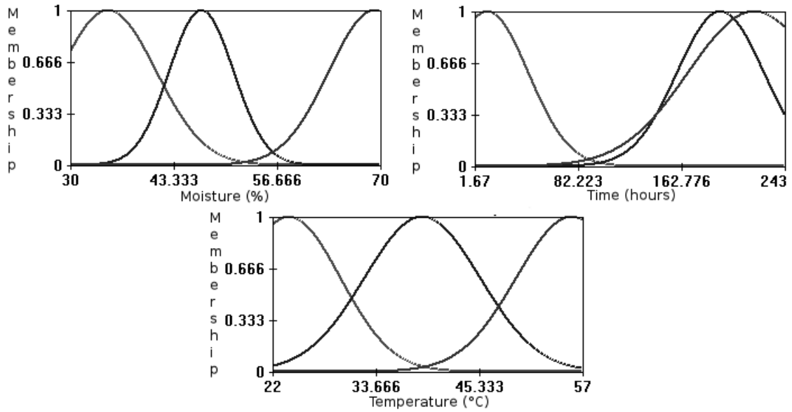
Figure 6.1: Membership functions, clockwise from top left: moisture, time, and temperature.
