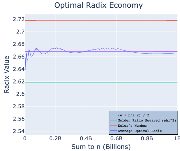
Figure 2.1.1: The above graph illustrates the empirically identified optimal radix value, \Omega , (blue line) given the associated limit n . The top and bottom horizontal lines (Euler's number (orange) and \phi^2 (green)) represent bases that are equidistant from the asymptotically defined optimal radix (purple line).
